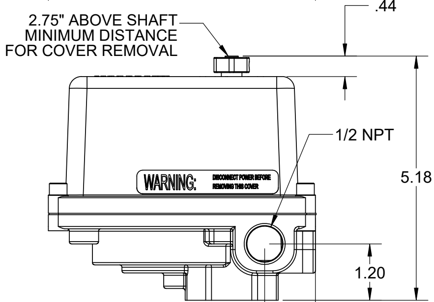
NEMA 4X ENCLOSURE
