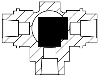
Open Position
