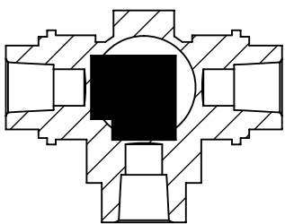
Closed Position
