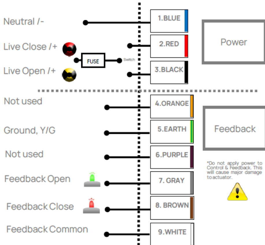
9P-5.08 Terminal diagram
